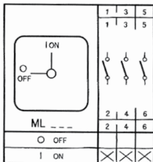
Contact Diagram 3-Pole
