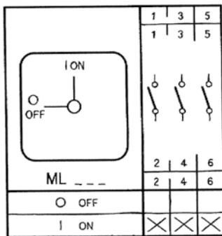
Contact Diagram 3-Pole
