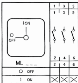
Contact Diagram 3-Pole
