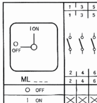
Contact Diagram 3-Pole
