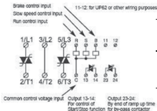
STL 3 3-phase configuration
