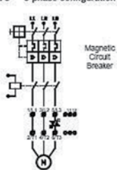
STL 3 3-phase configuration
