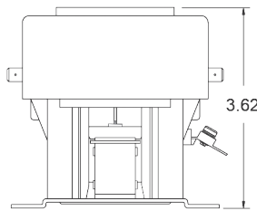
50 - 60 FLA Dimensions (inches) (weight = 2.0 lbs)
