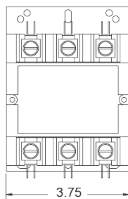
75- 90 FLA Dimensions (inches) (weight = 4.0 lbs)
