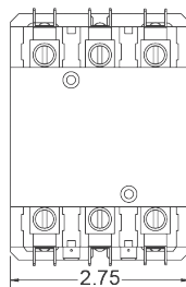
50 - 60 FLA Dimensions (inches) (weight = 2.0 lbs)
