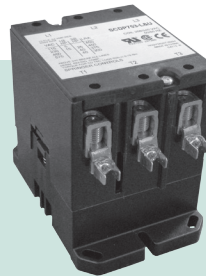
SCDP753-U6 75 amp, 3-Pole, 208-240V
